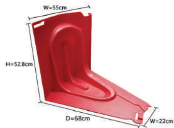
NW50 inner curved water retaining plate
