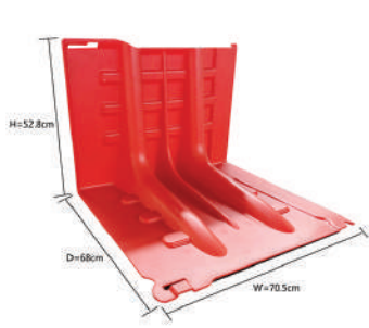
WZ50 straight water retaining plate
